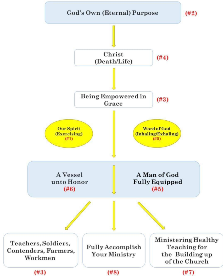
A Simple Diagram of 2024 Spring ITERO
